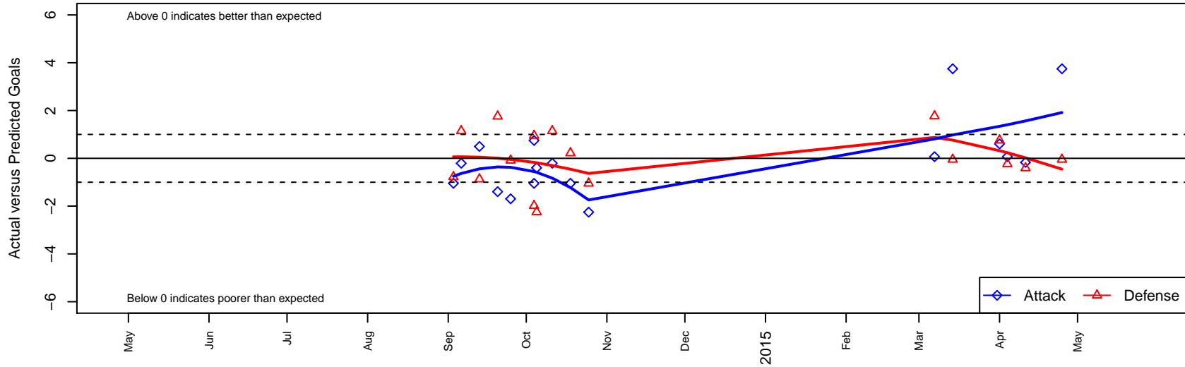
FC Nova White B03 Dots are actual minus expected GF (blue circles) and GA (red triangles). Blue line is smoothed change in attack strength. Red is smoothed change in defense strength.
